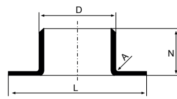
STUB END CURTA
