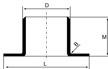
STUB END LONGA
